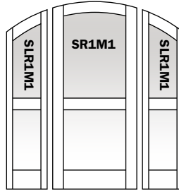
2 3 / 8 " stiles 4 1 / 16 " stiles 4 1 / 16 " top rail 4 1 / 16 " top rail 8" bottom rail 8" bottom rail
